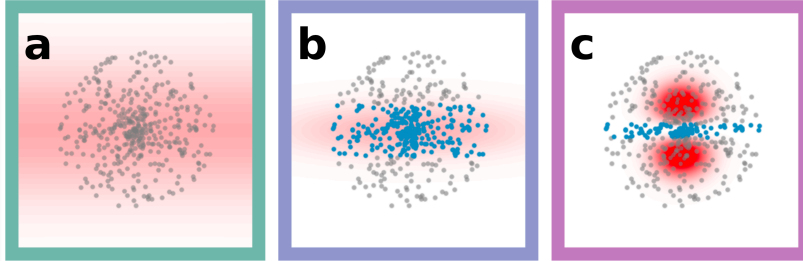
Figure 4.5: Cloud Slicing Sequence. (a) A large ( 500 \mu\text{m} waist) depump beam is shined on the atoms and depumps them to the |F = 1\rangle ground state. This beam is on resonance with the |F = 2\rangle \rightarrow |F' = 2\rangle transition. (b) A long vertical repump beam is switched on next, resonant with the |F = 1\rangle \rightarrow |F' = 2\rangle transition. This beam is narrow in the resonator axis to only repump atoms in the center of the cloud. (c) A \text{TEM}_{10} like slicing beam is turned on, tuned to the |F = 2\rangle \rightarrow |F' = 2\rangle transition. The node of the mode is aligned with the center of the cloud and spatially coincides with the resonator waist. After the slicing sequence, the cloud length is reduced to \sim 10 \mu\text{m} . Gray atoms represent the |F = 1\rangle groundstate and blue atoms represent the |F = 2\rangle groundstate.
