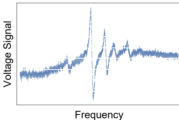
Figure 4.3: MOT locking signal . This signal is obtained by demodulating the Doppler-free spectrum of an enriched ^{87}\text{Rb} cell. The largest feature is the F = 2 \rightarrow F' = 2/F' = 3 crossover, located in frequency halfway between the F = 2 \rightarrow F' = 2 and F = 2 \rightarrow F' = 3 transitions. The MOT is locked to the zero crossing of the feature's downward slope.
